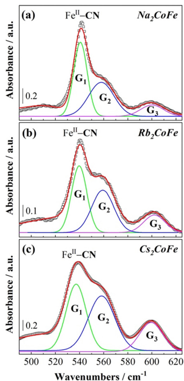
Fig. 7 Spectral deconvolution of (a) Na 2 CoFe , (b) Rb 2 CoFe and (c) Cs 2 CoFe over the 500–630 cm -1 range at 14 K. The open squares represent the experimental points and the solid lines the Gaussian fitting curves.
