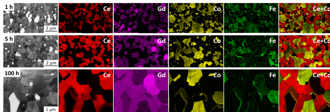
Fig. 6 Energy-filtered TEM (EFTEM) analysis of 60CGO20–FCO composite sintered at 1200 ^{\circ}\text{C} for 1 h, 5 h and 100 h, identifying three main phases: Gd-doped ceria (red), Fe/Co-oxide (green) and the \text{GdFeO}_3 -based perovskite (bright magenta).
