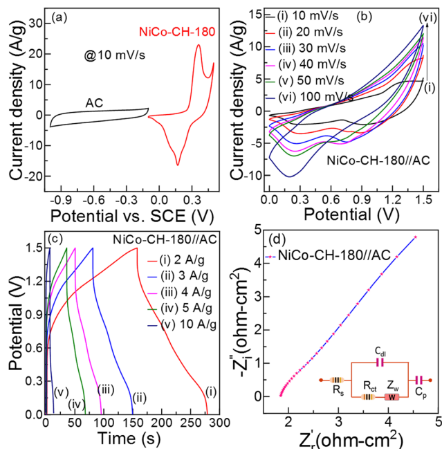
Fig. 6 (a) CV curve of the negative (AC) and positive (NiCo-CH-180) electrode at 10 \text{ mV s}^{-1} in a three-electrode set up, (b) CV curves for the ASC at various scan rates ( 10\text{--}100 \text{ mV s}^{-1} ), (c) GCD curves at different current densities ( 2\text{--}10 \text{ A g}^{-1} ), and (d) Nyquist plot of the NiCo-CH-180//AC ASC (two-electrode device).
