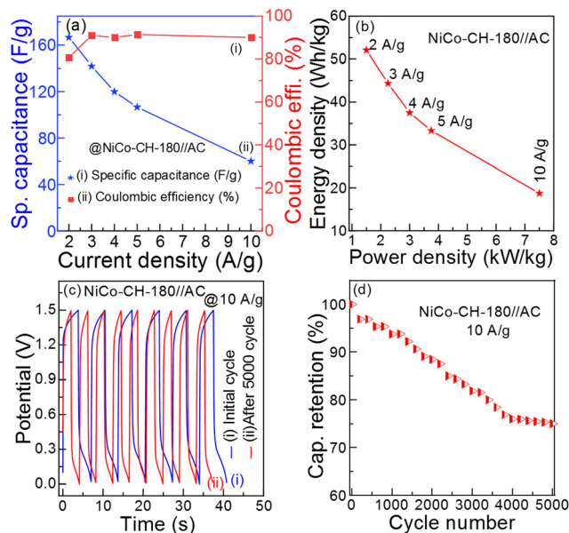
Fig. 7 (a) Specific capacitance and coulombic efficiency of NiCo-CH-180//AC ASC at different current densities ( 2\text{--}10 \text{ A g}^{-1} ), (b) Ragone plot (ED vs. PD), (c) initial and after 5000 charge-discharge curves, and (d) capacitance retention performance up to 5000 charge-discharge cycles at 10 \text{ A g}^{-1} current density of the NiCo-CH-180//AC ASC.
