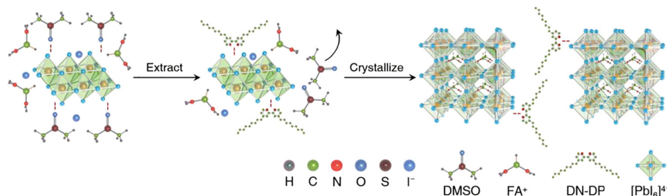
Fig. 6 The influence of DN-DP on the formation of the perovskite film. First, DN-DP exchange with DMSO to forms a new adduct of DN-DP– \text{PbI}_2 following the extension of the \text{PbI}_2 lattice. Then FA ions were inserted into the layered \text{PbI}_2 and exchanged with DN-DP. 126 The coordination between DN-DP and \text{PbI}_2 can retard the fast reaction between organic ammonium halides and \text{PbI}_2 , thus slowing down the crystallization rate and ensuring large grain growth. DN-DP reduces the residual DMSO in perovskite film, optimizes the contact of the buried interface, passivates the defects and changes the energy level, and finally improves the performance of the device. Reproduced from ref. 125 with permission from Elsevier, copyright 2023.
