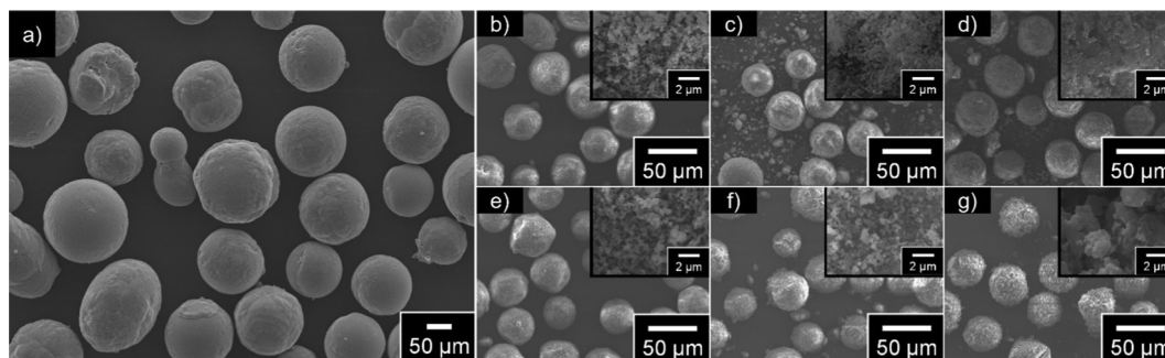
Fig. 2 SEM images of the MEPCMs before and after the treatment. (a) Raw material, (b) hybridized-PCM-alumina, (c) hybridized-PCM-alumina-ALOHH, (d) hybridized-PCM-ALOHH (e) MEPCM-alumina, (f) MEPCM-alumina-ALOHH, and (g) MEPCM-ALOHH. MEPCMs in (e)–(g) were derived by heat oxidation treatment of the corresponding HIB-treated MEPCMs from (b)–(d) at 1000 °C for three hours.
