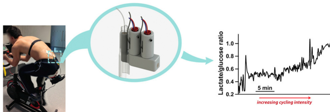
Fig. 2 A microfluidic system that measures lactate and glucose levels in dialysate during cycling. 60 Copyright 2015 American Chemical Society.
