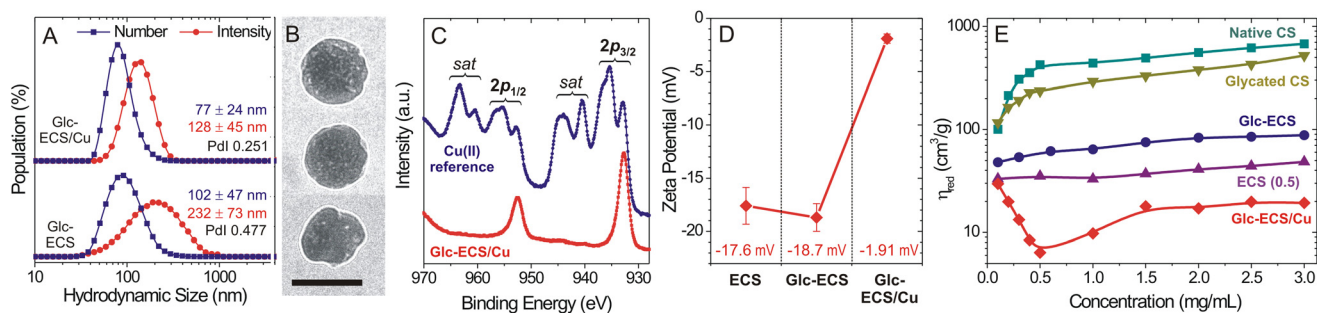
Fig. 5 (A) Hydrodynamic size distribution of Glc-ECS before and after the Cu(II) chelation. (B) TEM image of Glc-ECS/Cu (scale bar = 100 nm). (C) XPS analysis of the Cu 2p region in Glc-ECS/Cu. \text{CuSO}_4 was measured with Cu(II) as a reference and 'sat' indicates the satellite peaks in Cu(II). (D) Zeta potentials of ECS, Glc-ECS, and Glc-ECS/Cu measured at pH 7.0. (E) Viscosity analysis of CS derivatives measured in 20 mM acetate buffer (pH 4.0) containing 100 mM NaCl at room temperature.
