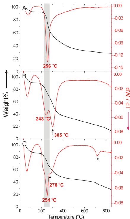
Fig. 4 TGA thermogram and differential thermogravimetric (DTG) curves of (A) glycosylated CS, (B) Glc-ECS, and (C) Glc-ECS/Cu. Asterisk at 718 °C indicates the decomposition of residual sulfate ions from CuSO 4 .
