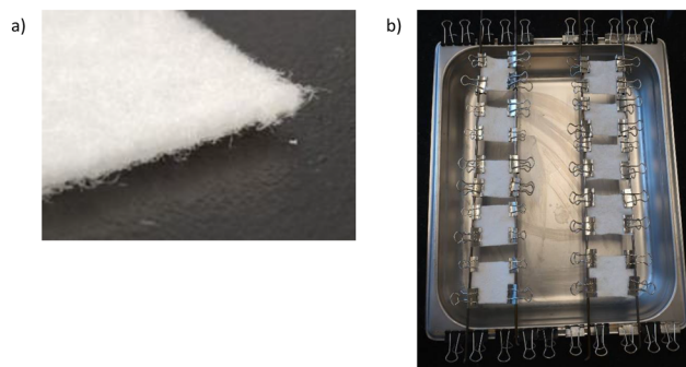
Fig. 2 (a) Image of PP fiber filtration felt and (b) assembly for the deposition of PEI and alkylated PEI derivatives at a concentration of 1 \times 10^{-4} \mu\text{mol N} per \text{cm}^2 .
