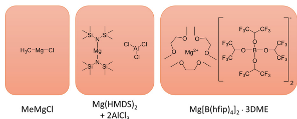
Fig. 1 Structures of the \text{MeMgCl} , \text{Mg}(\text{HMDS})_2\text{-}2\text{AlCl}_3 and \text{Mg}[\text{B}(\text{hfip})_4]_2\cdot 3\text{DME} electrolytes. In the case of \text{Mg}(\text{HMDS})_2\text{-}2\text{AlCl}_3 electrolyte, only the precursors are drawn, as a complex Schlenk equilibrium unfolds upon dissolving in a respective solvent. A detailed investigation of this behaviour was performed by Merrill and Schaefer. 18
