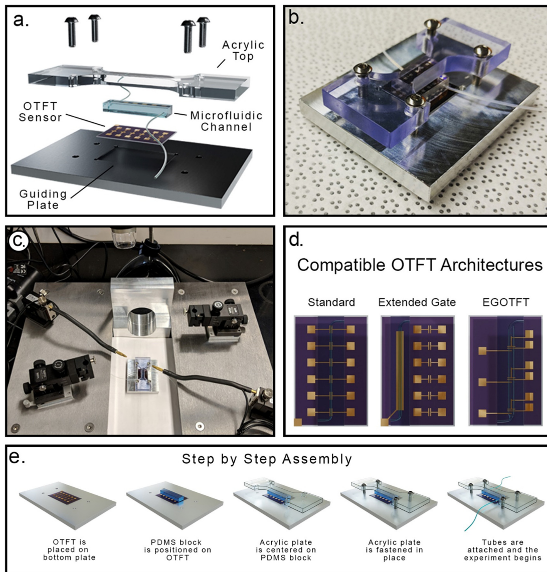
Fig. 1 Microfluidic OTFT pressure coupling system. (a) Schematic overview of the system components, (b) the assembled system with an OTFT, (c) assembled setup ready for testing. (d) Examples of compatible OTFT architectures (e) step by step assembly of the experimental setup.
