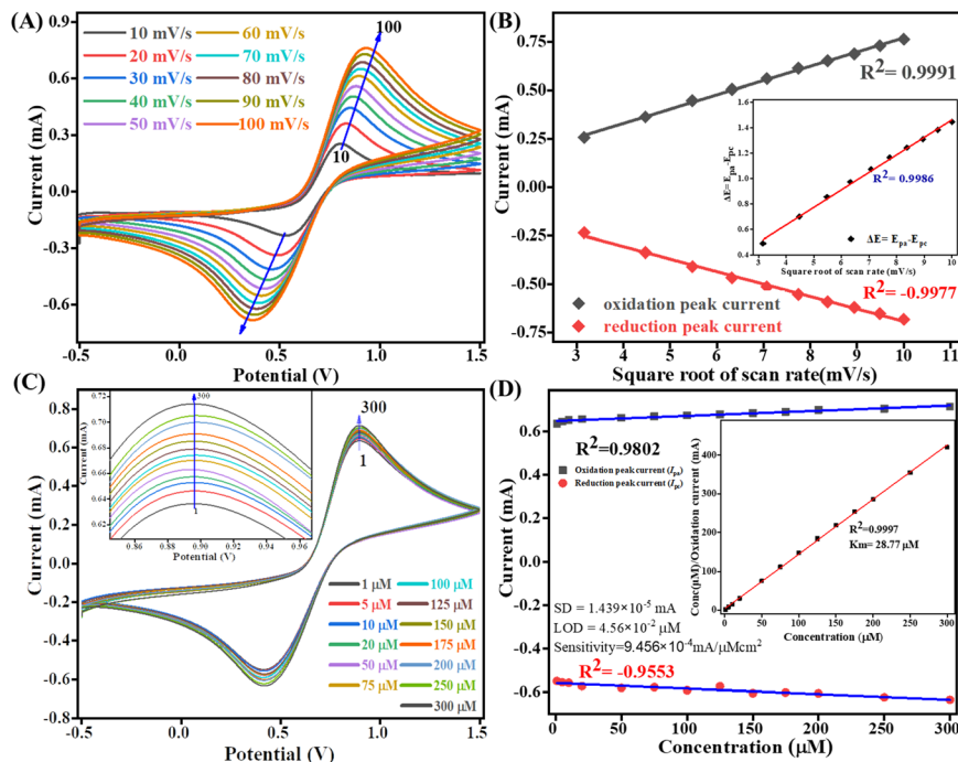
Fig. 9 Scan-rate analysis of (A) Tyr/Pg-NiFe 2 O 4 /rGO/ITO bioelectrode at 10–100 mV s -1 . (B) Linear-fit calibration curve of the square root of the scan rate (v 1/2 ) vs. peak current of the redox reaction. The inset image reveals the linear-fit curve between v 1/2 and ΔE (quasi-reversible nature of the bioelectrode). (C) Electro-oxidation of DA at a linear range of 1–300 μM. (D) Concentration linear-fit curve of DA at 1–300 μM, and the inset image shows determination of the Michaelis–Menten constant (K m ).
