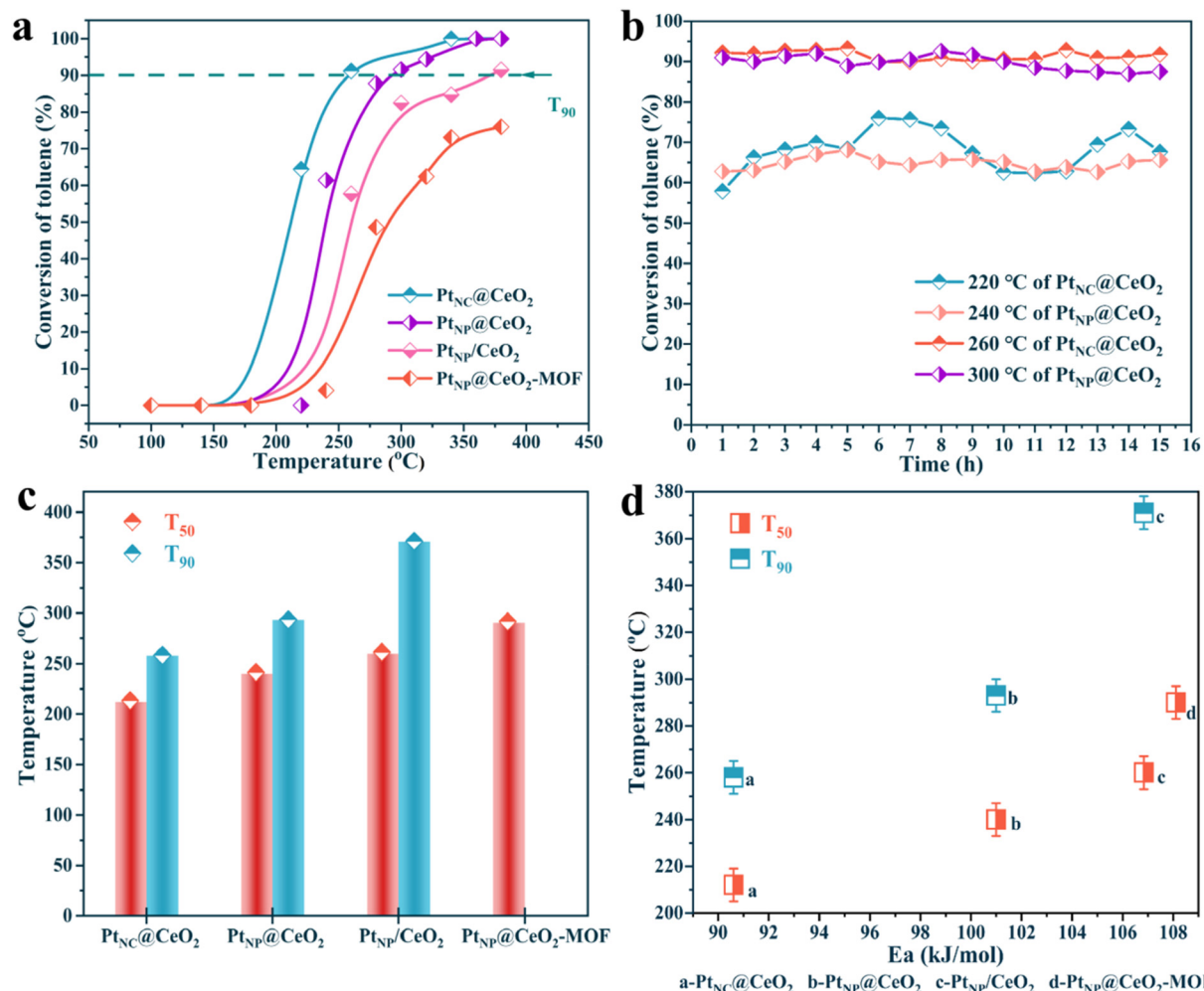
Fig. 1 The activity plot of Pt_{NC}@CeO_2 , Pt_{NP}@CeO_2 , Pt_{NP}/CeO_2 and Pt_{NP}@CeO_2-MOF catalysts (a), the stability tests of Pt_{NC}@CeO_2 and Pt_{NP}@CeO_2 under dry conditions (b), the comparison of T_{50} and T_{90} of each catalyst (c) and the catalytic activity versus E_a over the catalysts (d).
