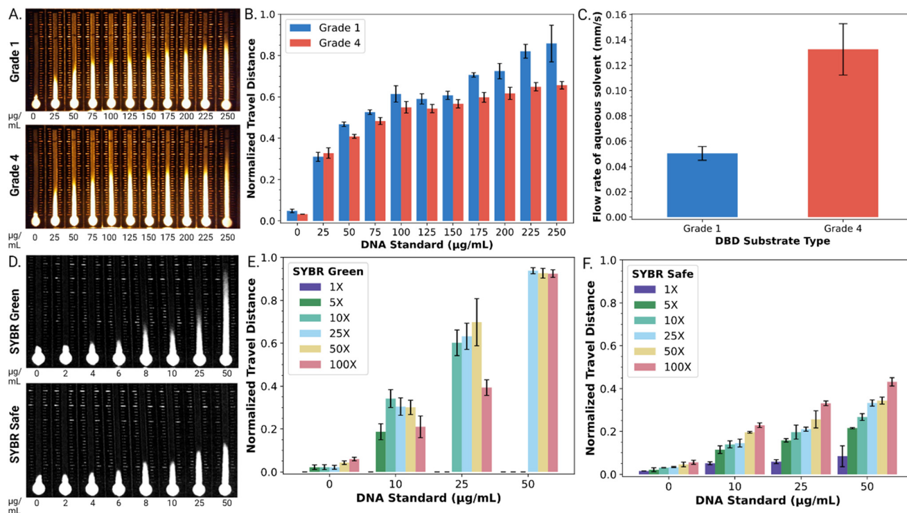
Fig. 2 Optimization of distance-based detection of dsDNA. A. Representative fluorescent images of dsDNA standards (0 to 250 \mu\text{g mL}^{-1} ) in grade 1 (top) and grade 4 (bottom) Whatman™ paper DBD substrates using 100 \times SYBR® Safe intercalating dye. B. Graph of normalized travel distance as a function of concentration of dsDNA in grade 1 (blue) and 4 (red) substrates. C. Graph of flow rates observed in grade 1 (blue) and grade 4 (red) substrates for 10 \mu\text{L} 0.1% w/w T90R4 in distilled water. D. Representative fluorescent images (blue channel only) of dsDNA standards (0 to 50 \mu\text{g mL}^{-1} ) in DBD substrates after exposure to 100 \times SYBR® Green I (top) and SYBR® Safe (bottom) dyes. E and F. Plots of normalized travel distances as a function of dsDNA concentration for varying concentrations of SYBR® Green I (Fig. 2E) or SYBR® Safe (Fig. 2F) [1 \times – purple, 5 \times – dark green, 10 \times – light green, 25 \times – blue, 50 \times – yellow, and 100 \times – red]. Error bars represent 1 std. deviation for n = 3 replicates per condition.
