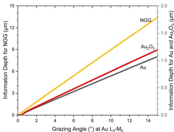
Fig. 3 Information depth at various exit angles for Au, Au_2O_3 , and NGG at Au L_3 - M_5 fluorescence line calculated from CXRO website 36 [last accessed 24.06.2024].
