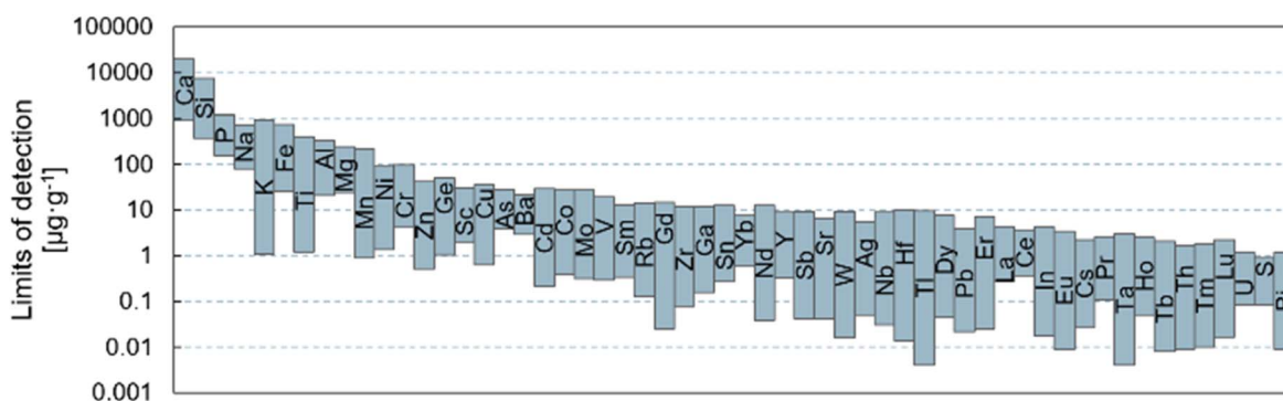
Fig. 2 Min–max range of limits of detection as obtained using LA-ICP-ToF-MS mapping of 0.004–0.05 mm 2 areas over a period of ~1 year. 2 µm ϕ circular, 3 µm ϕ circular, and 5 µm × 5 µm square laser spot sizes were used. Note that actual LoDs depend on multiple parameters other than the spot size. LoDs were calculated following Pettke et al. 20 Tuning of the mass analyzer may result in an improved sensitivity for the lower mass range, at the cost of sensitivity in the higher mass range.
