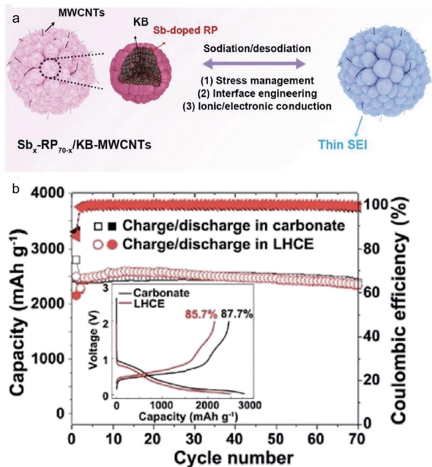
Fig. 13 (a) Schematic illustration and (b) cycling performance in carbonate electrolyte and localized highly concentrated ether electrolyte (LHCE) of hierarchical micro/nanostructured Sb_x\text{-RP}_{70-x}/\text{KB-MWCNTs} . Inset: first charge/discharge curve in two electrolytes. Reprinted with permission from ref. 125. Copyright 2021, American Chemical Society.
