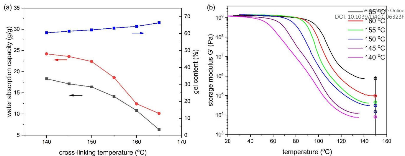
Figure 2. (a) Water absorption capacity and gel content of SAPs (all variations of SAP-80) versus cross-linking temperature; (■) water absorption capacity of unextracted SAP-80s (grinded for 180 s), (●) water absorption capacity of extracted SAP-80s (grinded for 180 s); (■) gel content of extracted SAP-80s (grinded for 180 s); note: All the data shown in the figure are average values based on the results obtained for three separate measurements and the margins of error are \pm 2 g/g for water absorption capacity test and \pm 0.2\% for gel content test. (b) Storage modulus as a function of temperature of extracted SAP-80s cross-linked at different temperatures (140 °C to 165 °C) for 1 h versus temperature, and grinded for 180 s. Note: 150 °C (vertical black line) was chosen as the point where G' was taken; since all curves reached a plateau before 150 °C it is reasonable to predict the G' value according to the existing curve. The circles are the predicted point at 150 °C
