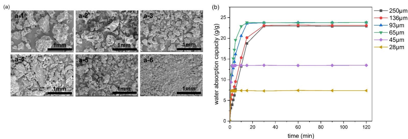
Figure 3. (a) SEM images of cross-linked (at 140 °C) and extracted SAP-80 particles grinded for different times (30, 60, 120, 150, 180, 210 s, respectively); (b) Plot of water absorption capacity versus swelling time (samples: cross-linked (at 140 °C) and extracted SAP-80, grinded to D_{circle\ equivalent} values of 250, 136, 93, 65, 45 and 28 \mu\text{m} obtained after grinding times varying from 30 to 210 s, respectively).
