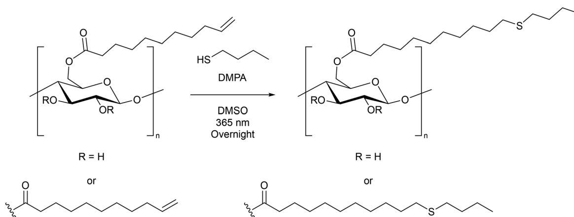
Scheme 10 An example of a thiol-ene reaction performed on a cellulose fatty acid derivative. 75
