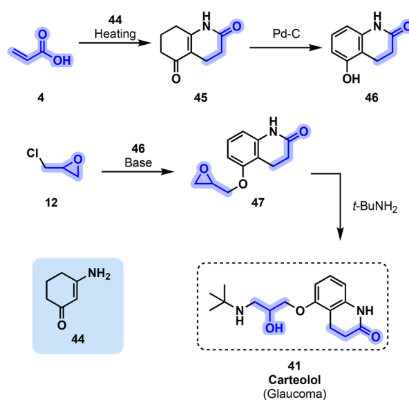
Fig. 9 Preparation of beta-blocker 41 , highlighting the incorporation of acrylic acid ( 4 ) and epichlorohydrin ( 12 ).
