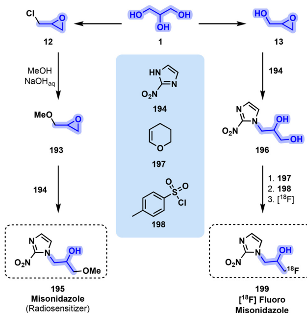
Fig. 40 Diverging pathways leading to misonidazole ( 195 ) and [ 18 F] fluoromisonidazole ( 199 ) from glycerol-derived epichlorohydrin ( 12 ) or glycidol ( 13 ).
