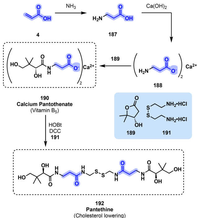
Fig. 39 Preparation of calcium pantothenate ( 190 ) and its dimeric form pantethine ( 192 ) from acrylic acid ( 4 ). HOBT = hydroxybenzotriazole, DCC = dicyclohexylcarbodiimide.
