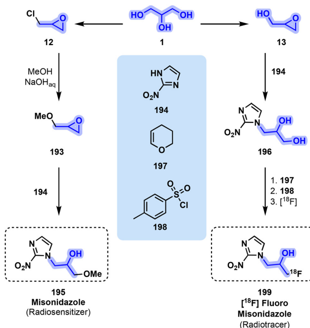
Fig. 40 Diverging pathways leading to misonidazole ( 195 ) and [ 18 F] fluoromisonidazole ( 199 ) from glycerol-derived epichlorohydrin ( 12 ) or glycidol ( 13 ).
