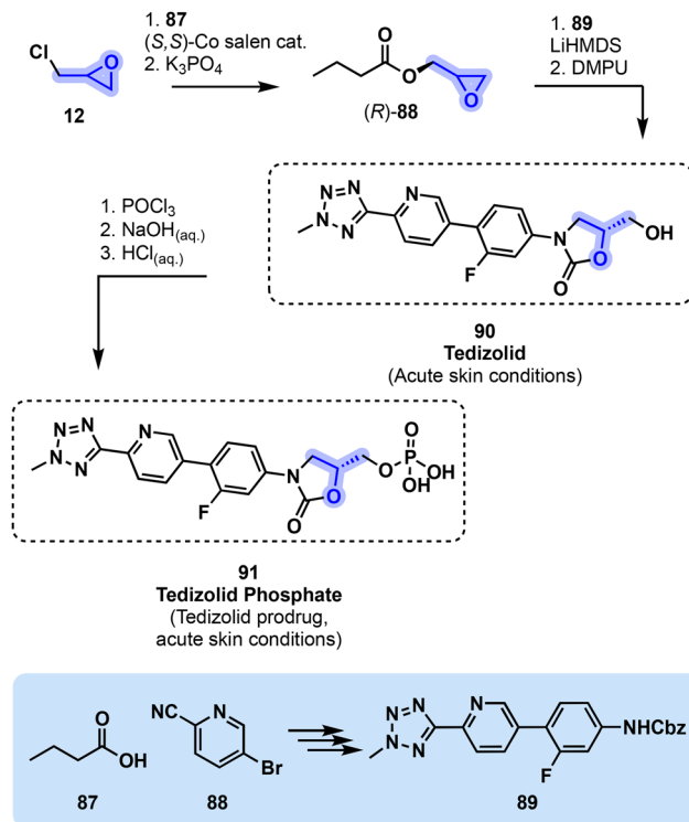
Fig. 20 Process-scale synthesis of tedizolid ( 90 ) and its phosphate prodrug 91 involving epichlorohydrin ( 12 ). LiHMDS = lithiumbis(trimethylsilyl)amide, DMPU = N,N' -dimethylpropyleneurea.
