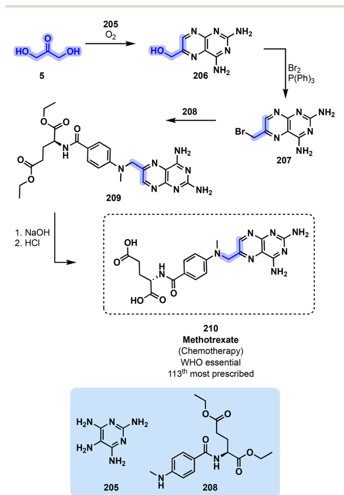
Fig. 42 Preparation of methotrexate ( 210 ) incorporating bio-based 1,3-dihydroxyacetone ( 5 ) and glutamic acid derivative ( 208 ).
