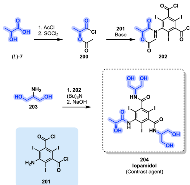
Fig. 41 Synthetic pathway leading to contrast agent iopamidol ( 204 ) incorporating two different glycerol derivatives: L-lactic acid ((L)-7) and 2-aminoglycerol ( 203 ).
