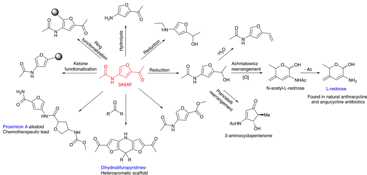
Scheme 3 Potential chemical transformation of 3A5AF.
