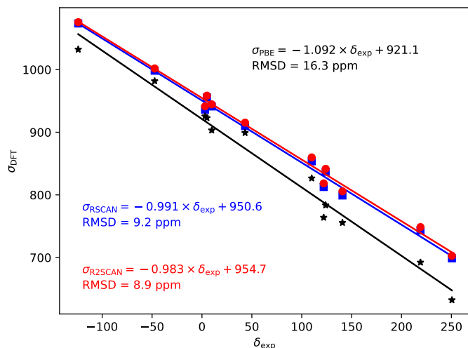
Fig. 4 ^{35/37}\text{Cl} magnetic shieldings, \sigma calculated with the PBE (black), rSCAN (blue) and r 2 SCAN (red) functionals vs. experimental chemical shifts, \delta . For each functional the line of best fit is given.
