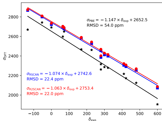
Fig. 5 ^{79/81}\text{Br} magnetic shieldings, \sigma calculated with the PBE (black), rSCAN (blue) and r 2 SCAN (red) functionals vs. experimental chemical shifts, \delta . For each functional the line of best fit is given.
