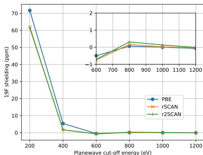
Fig. 1 Convergence of the ^{19}\text{F} magnetic shielding in \text{MgF}_2 with size of the plane-wave basis. Shieldings are given relative to the value at 1600 eV. The inset figure shows the close-up of the range from 600-1200 eV.
