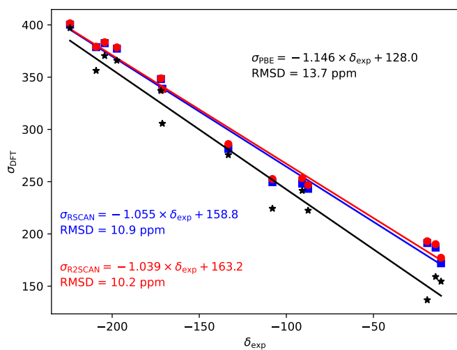
Fig. 2 ^{19}\text{F} magnetic shieldings, \sigma calculated with the PBE (black), rSCAN (blue) and r^2\text{SCAN} (red) functionals vs. experimental chemical shifts, \delta . For each functional the line of best fit is given.
