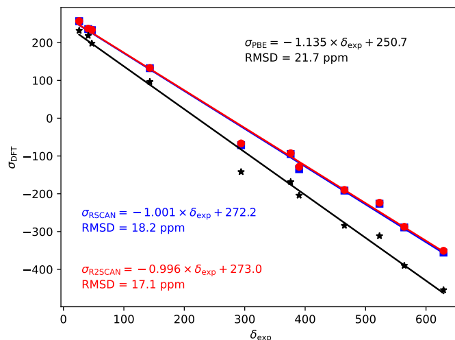
Fig. 3 ^{17}\text{O} magnetic shieldings, \sigma calculated with the PBE (black), rSCAN (blue) and r^2\text{SCAN} (red) functionals vs. experimental chemical shifts, \delta . For each functional the line of best fit is given.
