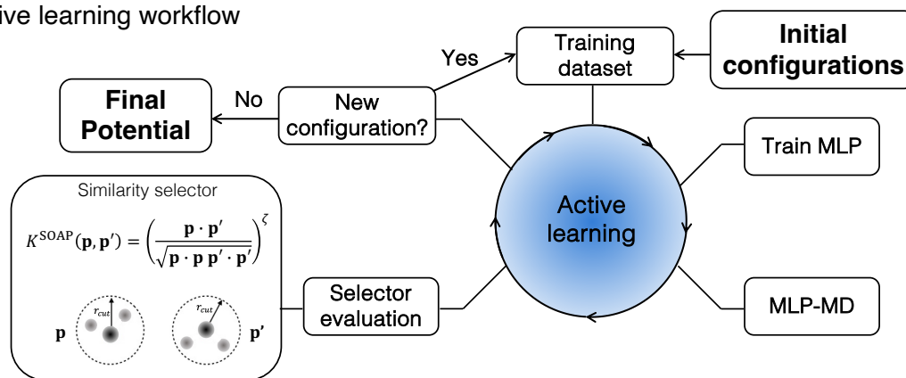
Fig. 1 Training data and active learning workflow: a) Training subsets for Mg 2+ in aqueous solution, b) training subset for Pd 2+ in acetonitrile (MeCN), c) Scheme of the active learning workflow used to train the machine-learning potentials (MLPs).
