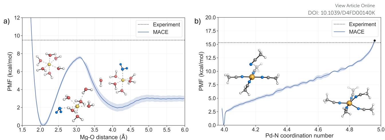
Fig. 4 Potential of mean force (PMF) profiles of the two ligand exchange processes for a) [\text{Mg}(\text{H}_2\text{O})_6]^{2+} (the solvent molecule exchanged is coloured blue) and b) [\text{Pd}(\text{MeCN})_4]^{2+} , where the black dot indicates the energy at the TS.
