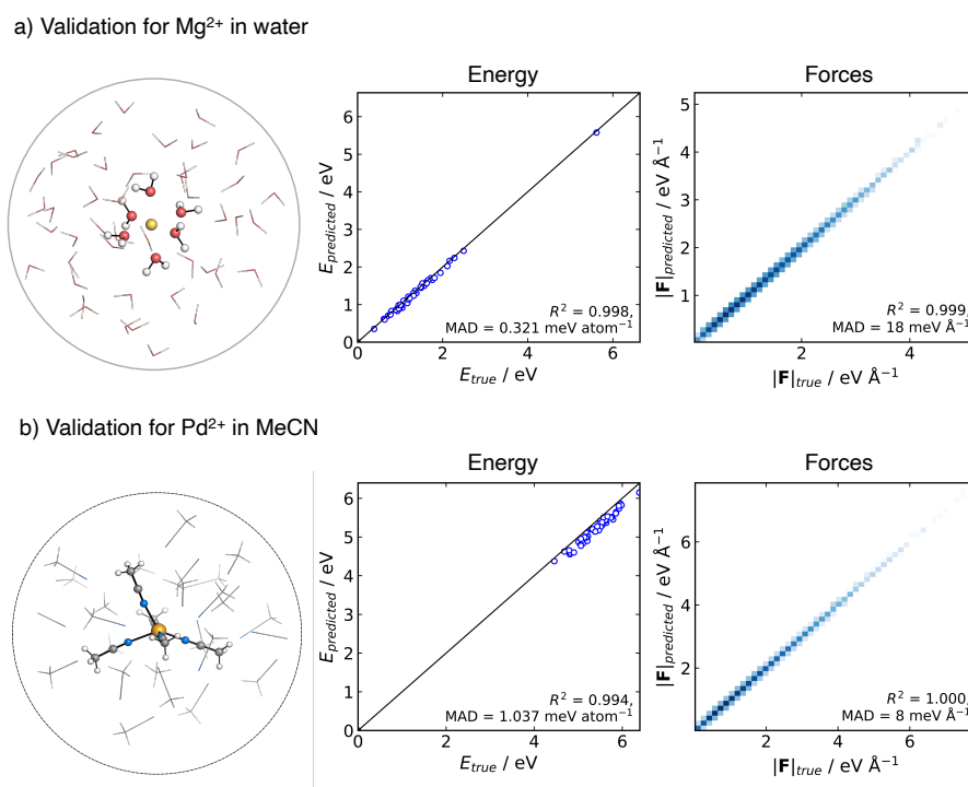
Fig. 2 Comparison of the ground-truth and MACE prediction of energies and forces for cluster systems at 300 K: a) \text{Mg}^{2+} solvated in 51 water molecules modelled at \omega\text{B97X-D3BJ}/\text{def2-TZVP} level of theory, b) \text{Pd}^{2+} solvated in 30 MeCN molecules modelled at \text{TPSS0-D3BJ}/\text{def2-TZVP} level of theory.
