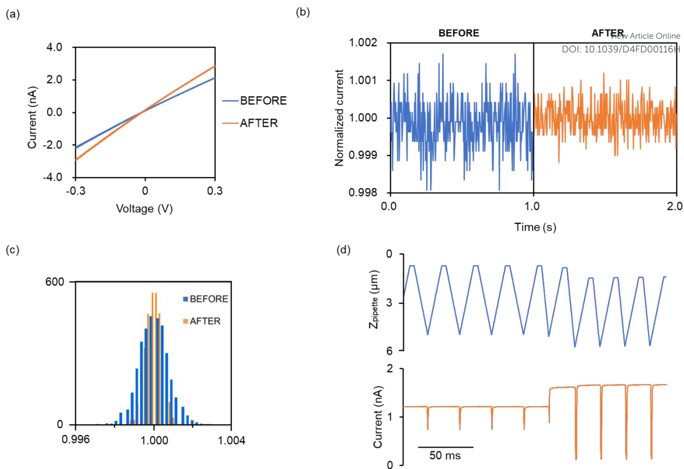
Figure 2. Nanopipette characterization. (a) Current–voltage characteristics, (b) chronoamperometry, and (c) a histogram before and after widening the nanopipette. (d) Traces of the nanopipette z position and pipette current during the widening procedure.
