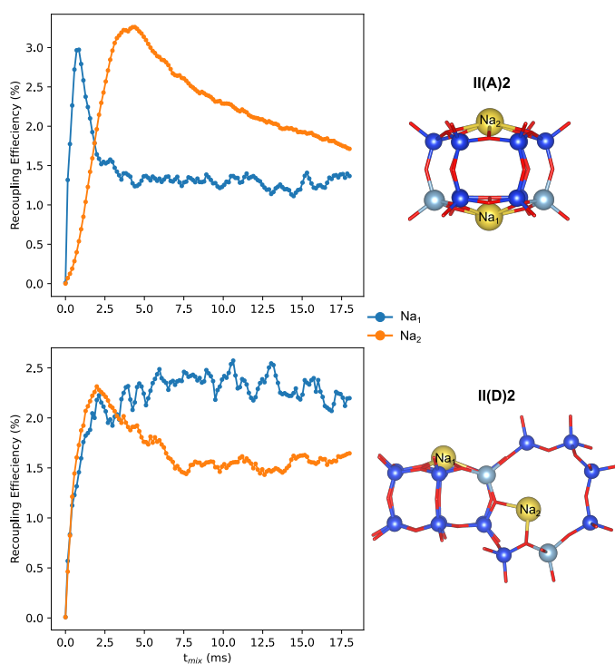
Fig. 5 Computed 23 Na- 27 Al recoupling build-up curves and respective structures
