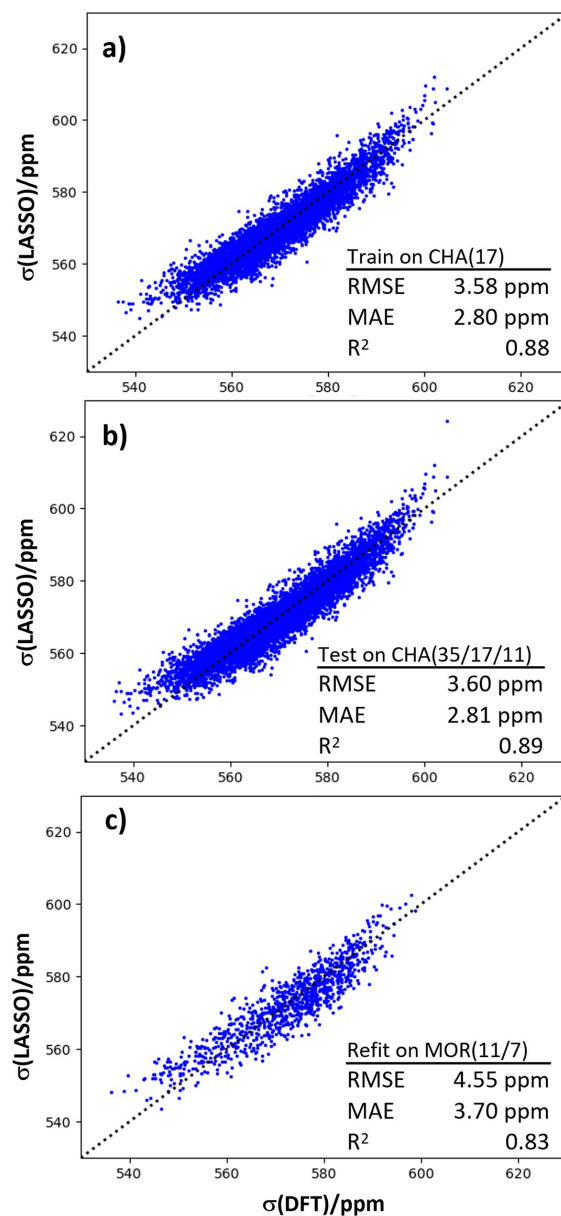
Fig. 6 a) Validation of the LASSO regression model against the training set of ^{23}\text{Na} chemical shifts of CHA(17) configurations, b) Generalization test of the LASSO model against CHA(35) and CHA(11) configurations, c) Performance of the retrained model against MOR(11) data.
