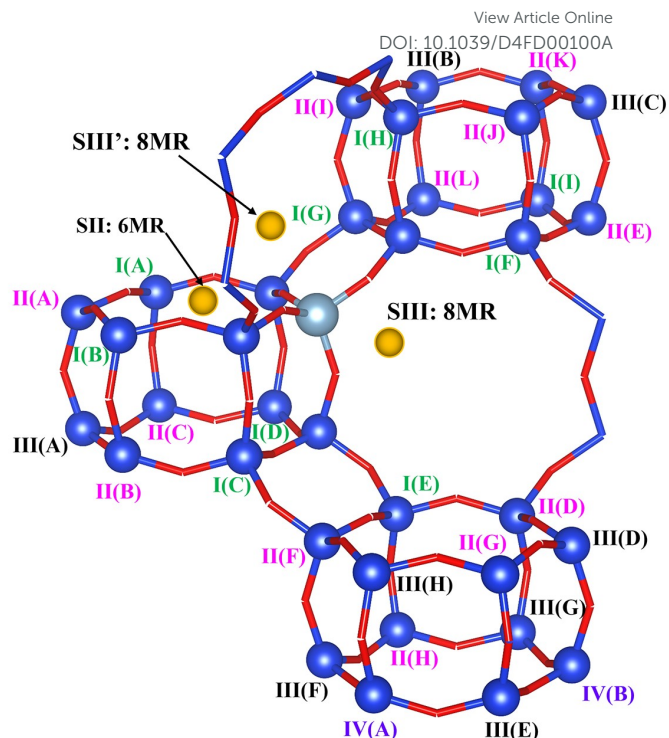
Fig. 1 Model for the 36 T site CHA zeolite used in this work. Labels for configurations in the CHA(17) model are given. The Al configurations are named with I/II/III/IV(x), where I, II, III and IV are used to denote the shortest Al-Si n -Al sequences with n = 1, 2, 3 and 4, respectively, and x are letters to distinguish the different sites with same n . The yellow balls denote the possible locations of \text{Na}^+ , SII is on the 6MR window and SIII is on the 8MR window as defined in the previous work 50
