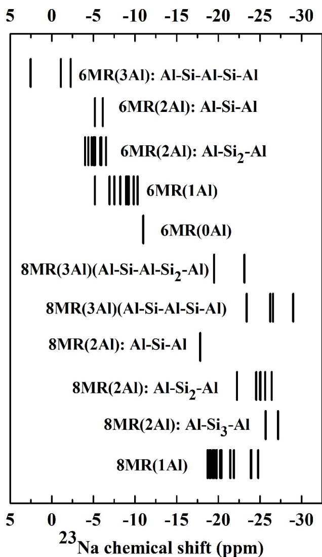
Fig. 3 DFT ^{23}\text{Na} isotropic chemical shift calculated from CHA(11) models.
