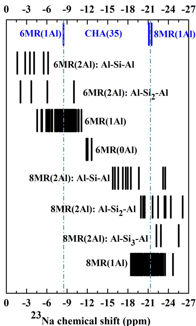
Fig. 2 DFT ^{23}\text{Na} chemical shifts calculated from all low energy local minima for CHA(X), (X = 35, 17) (shown in Figure S2 and S3).
