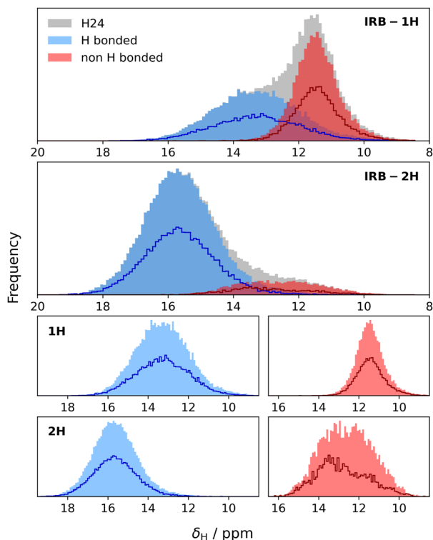
Fig. 6 ShiftML2-predicted chemical shifts of all tetrazole H atoms for IRB-1H and IRB-2H from 501 frames of MD simulations at 300 K. The H atoms are classified into hydrogen-bonded (blue) vs. non-hydrogen bonded (red) based on an angular cutoff of 125^\circ and distance cutoff of 3.5 Å. Darker outlines show the distribution of the chemical shifts for the corresponding components in the IRB-1H2H mixture. The four lower plots show each histogram separately for clarity.
