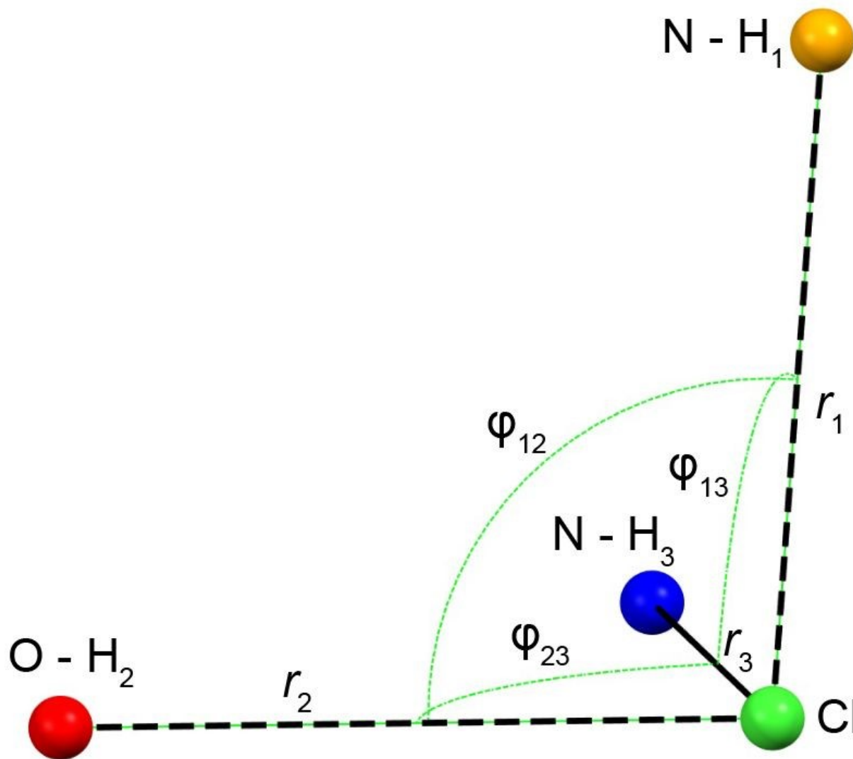
Figure 3. Schematic of the \text{H}\cdots\text{Cl} hydrogen bond network for the DFT-D2* refined crystal structures of Eph and Pse. From shortest to longest, r_1 , r_2 , and r_3 correspond to the \text{H}\cdots\text{Cl} bond lengths with secondary amine, alcohol, and another secondary amine moieties, respectively. Angles \varphi_{ij} describe the interbond angles. Values are shown in Table 3 .
