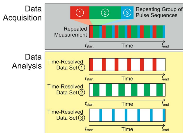
Fig. 2 Schematic of the CLASSIC NMR technique, illustrated for the case in which in situ NMR spectra are recorded as a function of time during crystallization by repeated measurement of a set of three pulse sequences (shown in red, green and blue) representing the "repeating group". After completing the experiment, the three sets of data are separated to give a set of time-resolved NMR spectra for each of the three pulse sequences.
