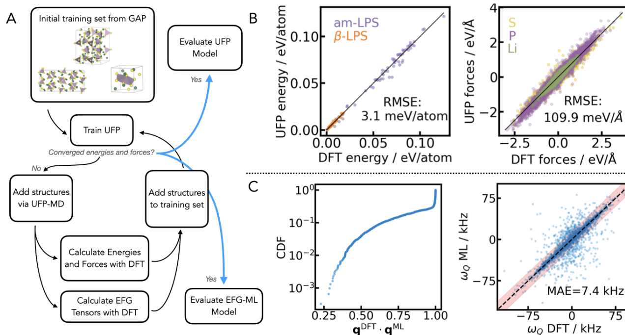
FIG. 1. Workflow of the UFP+ML-EFG training. The left panel shows the active learning workflow (A) starting from a set of structures used to train a GAP [28] for LPS [31] to the final training of the UFP (B) and ML-EFG model (C). The UFP has an RMSE in the energies of 3.1 meV/atom and forces of 109.9 meV/Å. The ML-EFG model is assessed both by the quality of the relative orientation of the tensors and the MAE in \omega_Q . C shows the combined distribution function (CDF) of the quaternion scalar product between the DFT and ML quaternions, \mathbf{q}^{\text{DFT}} \cdot \mathbf{q}^{\text{ML}} . This indicates that the majority of tensors are oriented in the same direction comparing DFT to ML. The ML-EFG model has an error of 7.4 kHz on \omega_Q , where the experimental sensitivity of ^7\text{Li} SAE is shown shaded in red, as 10 kHz for \omega_Q .
