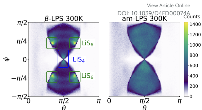
FIG. 6. Heatmap \theta and \phi distributions in \beta - and am-LPS. The heatmaps show the concentration of the angles \theta and \phi across the full 1 \mu\text{s} UFP-MD trajectory. The distributions are colored by the total number of sites with that combination of angles (\theta, \phi) , and in \beta -LPS the angle pairs which arise from \text{LiS}_4 and \text{LiS}_6 sites are indicated.
