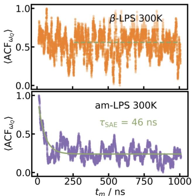
FIG. 3. \langle \text{ACF}_{\omega_Q} \rangle for \beta -LPS and am-LPS The \langle \text{ACF}_{\omega_Q} \rangle given by Equation 4 calculated over a 1 \mu\text{s} UFP-MD simulation at 300 K for 144 Li atoms in single-crystalline \beta -LPS (top, orange) and 216 Li atoms in am-LPS (bottom, purple). A decay time, \tau_{\text{SAE}} = 46\text{ns} can be extracted from the am-LPS \langle \text{ACF}_{\omega_Q} \rangle .
