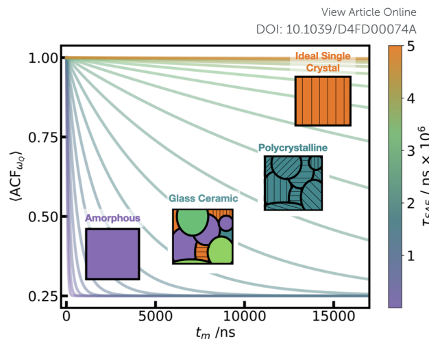
FIG. 7. Schematic of range of crystalline to amorphous \tau_{\text{SAE}} . The left shows a range of decay functions, Equation 5, with \tau_{\text{SAE}} from 50 ns to 5 million ns. The inset figures show schematics of the expected microscale structure at each of these varying decay rates, with black lines in the glass ceramic and polycrystalline denoting different grains.
