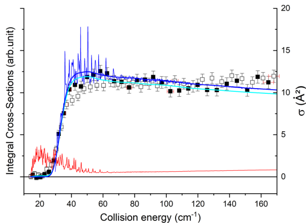
Fig. 8 Experimental and theoretical cross-sections for the HDO + Ne → HDO ( 1_{11} ) + Ne inelastic collisions. Squares are experimental ICSSs for the 1_{11} rotational level, with error bars corresponding to statistical uncertainties at 95% of the confidence interval (white or black squares are the means of around 7000 or 9200 data, respectively). Shown as solid lines, the total theoretical contributions are convoluted to the experimental collision-energy spread, with partial contributions of the 1_{11} \leftarrow 0_{00} transition (as a thin blue line) and the 1_{11} \leftarrow 1_{01} transition (as a thin red line), assuming an initial rotational population from the 1_{01} state of 0% (as a bold blue line) or 5% (as a bold cyan line).
