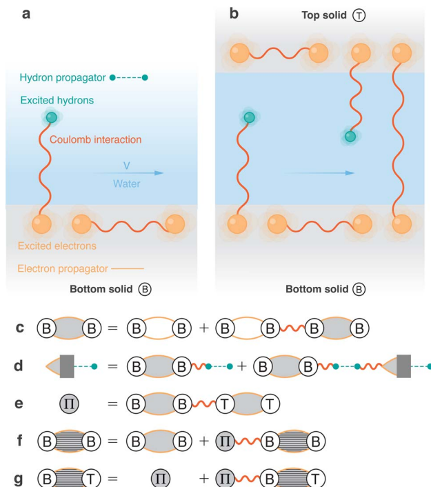
Fig. 4 Fluctuation-induced effects. (a) Schematic of the interactions involved in single-interface quantum friction. Friction results from the Coulomb coupling of liquid fluctuations (hydrons) and electronic fluctuations. (b) Schematic of the interactions involved in confined quantum friction. Compared to the non-confined case, there is an additional Coulomb interaction between the charge fluctuations in the two solid walls. (c) Dyson equation for the renormalization of the bottom wall's charge density response function (polarization "bubble") by the intra-wall Coulomb interactions. The bare bubble is empty and the renormalized bubble is filled with gray. (d) Dyson equation for the electron–water susceptibility \chi_{ew} . (e) Definition of the exchange term \Pi (see text). (f) Dyson equation for the renormalization of the bottom wall's charge density response function by the inter-wall Coulomb interactions. The stripes indicate a fully-renormalized bubble. (g) Dyson equation for the inter-wall charge density response function, which vanishes in the absence of inter-wall Coulomb interactions ( \Pi = 0 ).
