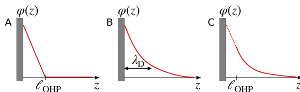
Fig. 1 Schematic electrical potential profiles in the EDL predicted by (A) Helmholtz–Perrin theory, (B) GC theory, and (C) GC theory with the Stern correction, where the dashed section represents the linear decay in the Stern layer.
