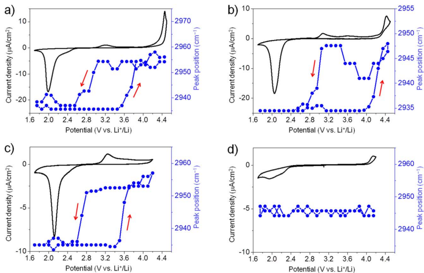
Fig. 3 Potential dependence of peak position of the SFG band around 2955\text{ cm}^{-1} (blue symbols) during ORR/OER. (a) \text{O}_2 -saturated 0.1 M LiTFSI/G2; (b) \text{O}_2 -saturated 0.1 M LiTFSI/G3; (c) \text{O}_2 -saturated 0.1 M LiTFSI/G4; (d) Ar-saturated 0.1 M LiTFSI/G4. CV curves are given for comparison (solid trace).
