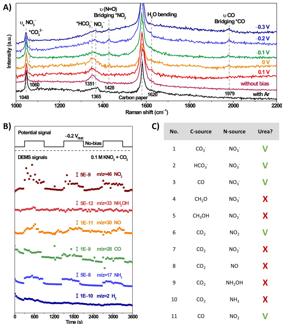
Fig. 16 Mechanistic investigations involving the formation of ^*\text{O}_2\text{NCO} using the \text{CuWO}_4 catalyst. (A) In situ Raman spectra at different potentials. (B) Online DEMS at -0.2 V vs. RHE. (C) Control experiment with various C- and N-sources. Adapted from ref. 188 (Open Access).
