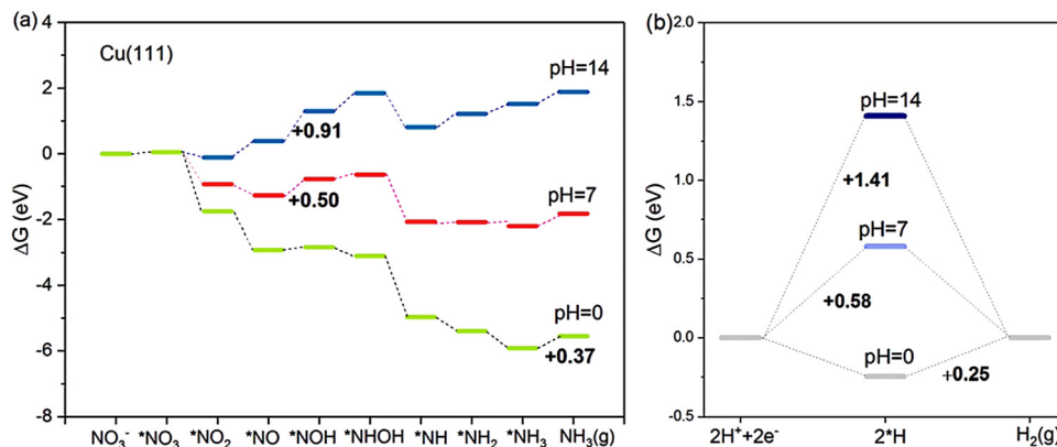
Fig. 4 The competition between (a) \text{NO}_3\text{RR} and (b) \text{HER} on Cu (111) at pH = 0, 7 and 14, studied by Hu et al. Reprinted with permission from ref. 33. Copyright 2021, American Chemical Society.
