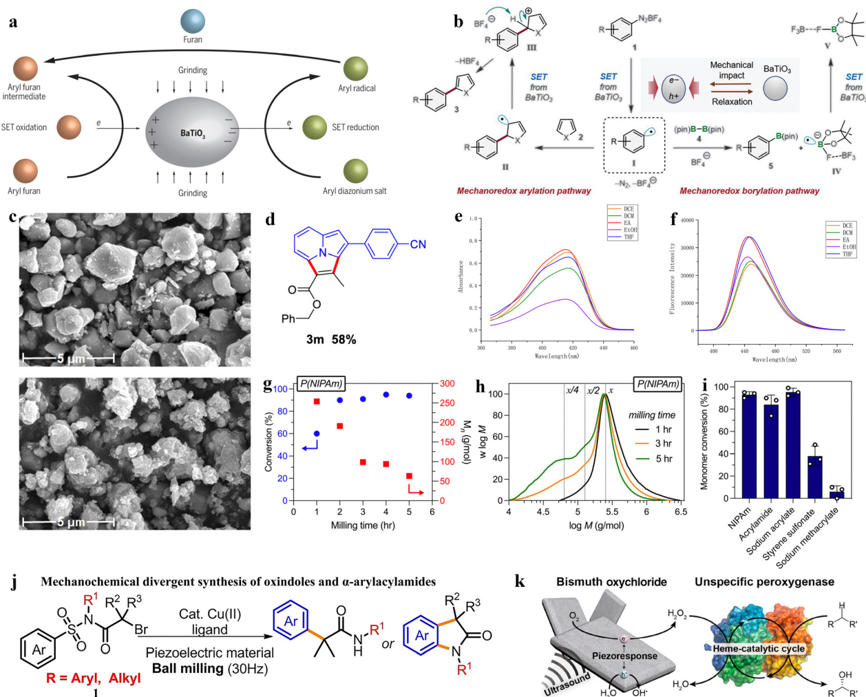
Fig. 7 (a) Grinding piezoelectric barium titanate ( BaTiO_3 ), aryl diazonium salt, and furan with a ball mill allows organic synthesis of aryl furan compounds. 121 Copyright 2019, The American Association for the Advancement of Science. (b) Proposed mechanism for the mechanoredox arylation and borylation using BaTiO_3 and ball milling. 125 Copyright 2019, The American Association for the Advancement of Science. (c) SEM of BaTiO_3 particles before and after fluorination. 127 Copyright 2023 Wiley-VCH GmbH. (d) Compound 3m (benzyl 3-(4-cyanophenyl)-2-methylpyrrolo[2,1,5- cd ]indolizine-1-carboxylate). (e) Ultraviolet-visible absorption spectra. (f) Fluorescence (excited at \lambda_{max} ) spectra of 3m . 129 Copyright 2022 American Chemical Society. (g) Monomer conversion values for a range of solid vinyl monomers through ball milling with BaTiO_3 . (h) Mechanochemical divergent syntheses of oxindoles and \alpha -arylacrylamides. (i) Schematic illustration of piezobiocatalytic oxyfunctionalization reactions by BiOCl -rAaeUPO Hybrida. 130 Copyright 2023 The Authors. Angewandte Chemie International Edition published by Wiley-VCH GmbH. (j) Mechanochemical divergent syntheses of oxindoles and \alpha -arylacrylamides. 131 Copyright 2022 Wiley-VCH GmbH. (k) Piezoelectric BiOCl microsheets induce piezocatalytic reduction of O_2 to H_2O_2 under ultrasonic irradiation. The in situ -generated H_2O_2 activates the redox center of an unspecific peroxygenase to catalyze selective oxyfunctionalization of various organic compounds. 132 Copyright 2020 American Chemical Society.
