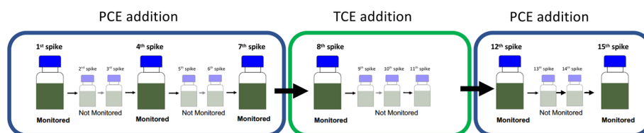
Fig. 1 Overview of the (re-)spike experiments of the synthetic binary culture containing Desulfitobacterium dehalogenans strain PCE1 and Desulfitobacterium hafniense strain Y51.
