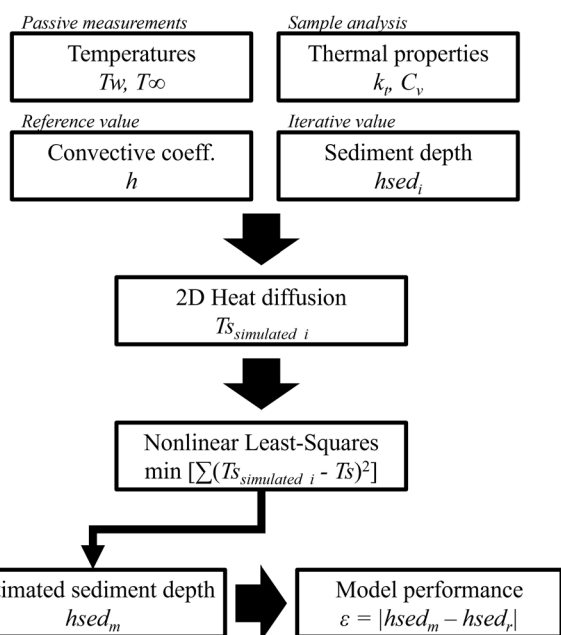
Fig. 3 Scheme to estimate sediment depths using the temperature-based model and evaluate its performance.
