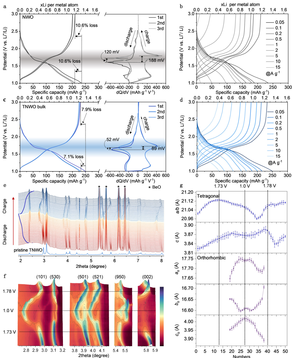
Fig. 3 Electrochemical \text{Li}^+ storage behaviors of NWO bulk and TNWO bulk anodes in coin-type half cells. (a) and (c) GCD curves at 0.05 \text{ A g}^{-1} and corresponding dQ/dV plots (Q: capacity; V: potential) for initial three cycles. (b) and (d) Initial GCD curves at current densities ranging from 0.05 \text{ A g}^{-1} to 15 \text{ A g}^{-1} . (e)–(g) Operando high-energy synchrotron XRD patterns and the corresponding GCD curve, contour plots and refined lattice parameter evolution during the initial (de)lithiation process of the TNWO bulk anode.
