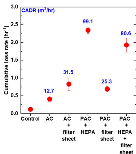
Fig. 10 Cumulative loss rate (CLR) of different mitigation techniques: (i) AC (without filter sheet), (ii) AC + filter sheet, (iii) PAC + HEPA, (iv) PAC + filter sheet, and (v) PAC + HEPA filter + filter sheet; CADR ( \text{m}^3 \text{ h}^{-1} ) is written on top of each compared technique.
