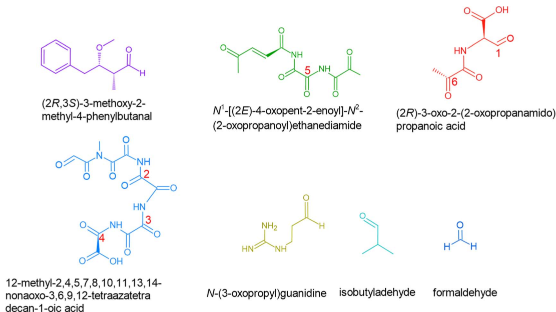
Fig. 3 Potential fragmentation products resulting from the degradation of MC-LR by reaction with \cdot\text{OH} and \text{O}_3 .
