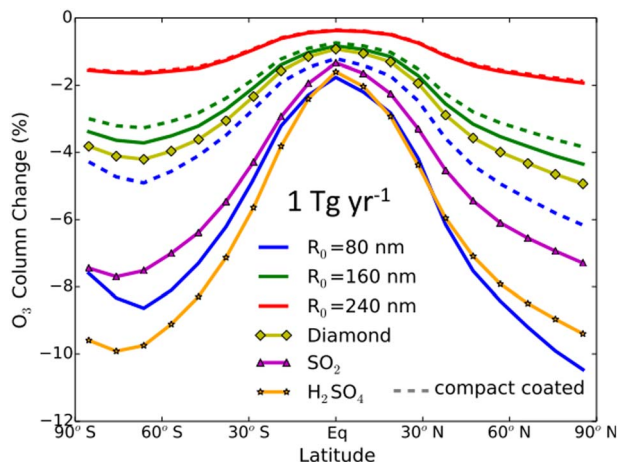
Fig. 9 Average O_3 column change per year as a function of latitudes with an annual injection rate of 1 \text{ Tg yr}^{-1} of Al_2O_3 monomers of 80 nm (blue), 160 nm (green), 240 nm (red), 160 nm diamond monomers (dark yellow), SO_2 (magenta), and H_2SO_4 (orange). Reprinted from Weisenstein et al. , Atmos. Chem. Phys. , 2015, 15, 11835–11859. Distributed under a Creative Commons Attribution 4.0 License (CC BY 4.0) https://creativecommons.org/licenses/by/4.0/ .
