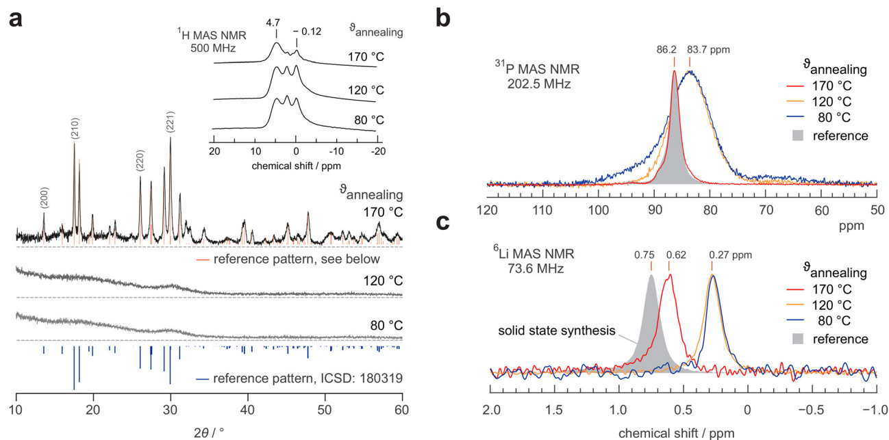
Fig. 1 (a) XRPD patterns of the \beta -Li 3 PS 4 precursor (bottom) and the samples annealed at 120 °C (middle) and 170 °C (top), respectively. Vertical bars shown at the very bottom indicate the reference pattern (ICSD: 180319) of \beta -Li 3 PS 4 . Values in brackets refer to the hkl indices. The inset shows the corresponding 1 H MAS NMR lines. (b) 31 P MAS NMR spectra (25 kHz spinning speed) of the samples annealed at the indicated temperatures \vartheta_{\text{annealing}} . For comparison, the corresponding spectrum of the mechanochemically prepared \beta -Li 3 PS 4 sample is shown in grey. 25 (c) 6 Li MAS NMR spectra (25 kHz) for the same samples as in (b); again, the sample obtained via the solid-state mechanochemical approach is indicated in grey. 25
