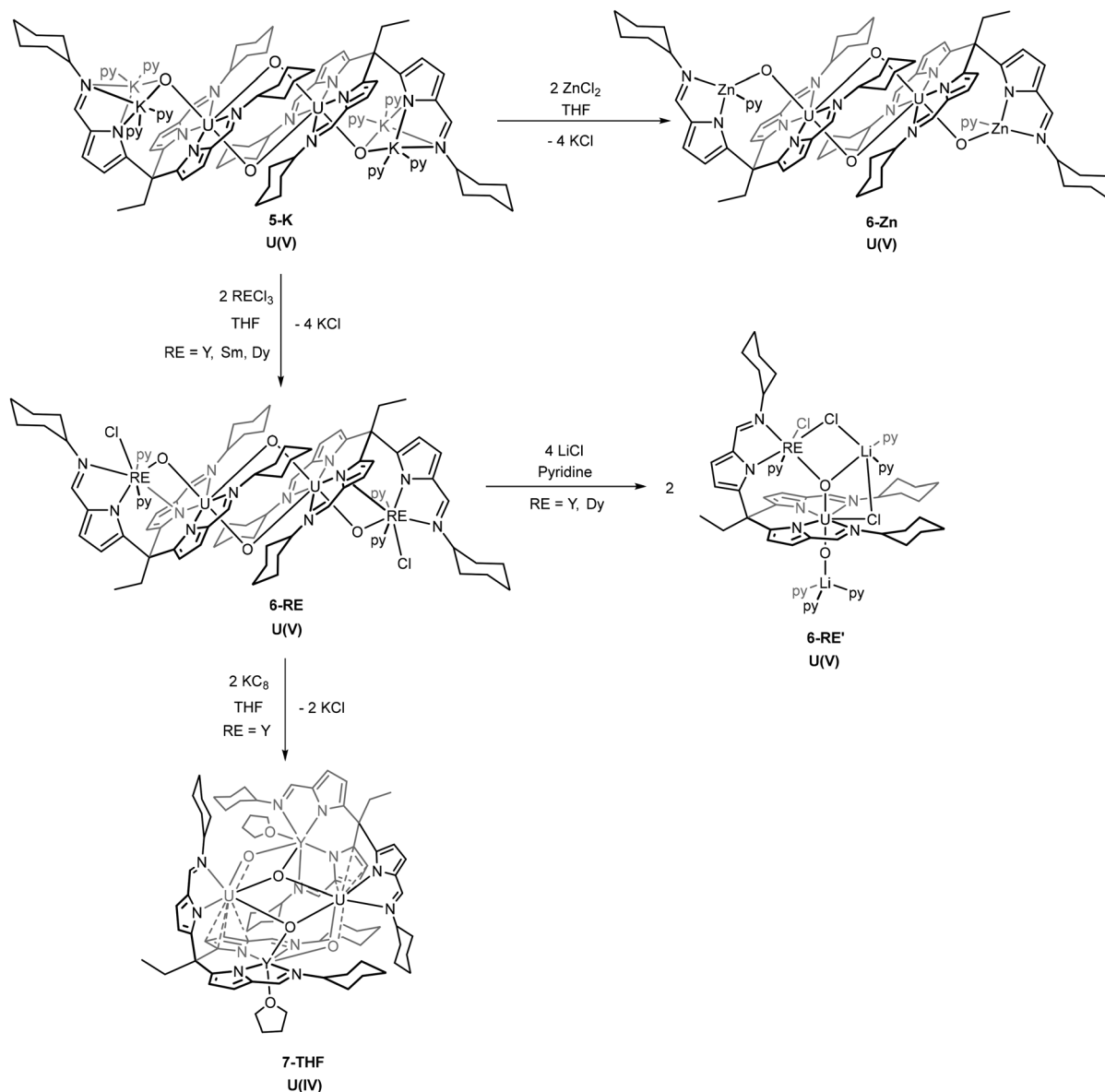
Scheme 3 Synthetic procedures to the formation of the U(v) heterobimetallic complexes [\text{UO}_2\text{Zn}(\text{L})_2] ( 6-Zn ), and [\text{UO}_2\text{RE}(\text{LCl})_2] ( 6-RE ) by reaction of 5-K with the respective metal chloride; [\text{UO}_2\text{RE}(\text{L})(\text{LiCl})_2] ( 6-RE' ) by the treatment of 6-RE with four equivalents of LiCl; and the dimeric U(IV) complex [\text{UO}_2\text{Y}(\text{L})(\text{THF})]_2 ( 7-THF ), by the reduction of 6-Y with two equivalents of \text{KC}_8 .
