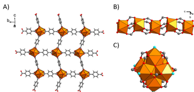
Fig. 9 Thorium–organic frameworks based BDC structures synthesized with (A) DMF: Th(BDC) 2 (DMF) 2 (B) H 2 O: Th(BDC) 2 (C) DMF and H 2 O: Th 6 O 4 (OH) 4 (H 2 O) 6 (BDC) 6 DMF 12 H 2 O. Reprinted with permission from Inorg. Chem. , 2015, 54 (5), 2235–2242. © 2015 American Chemical Society.
