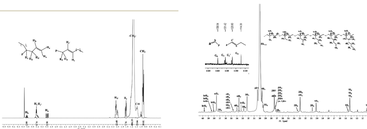
Fig. 10 ^{13}\text{C} NMR spectrum of the polyethylene sample produced using Ni5/EASC at 20 °C (entry 5, Table 4) together with an inset showing the \delta 114–140 region and a segment of the assigned polymer backbone recorded at 110 °C in 1,1,2,2-tetrachloroethane- d_2 .
