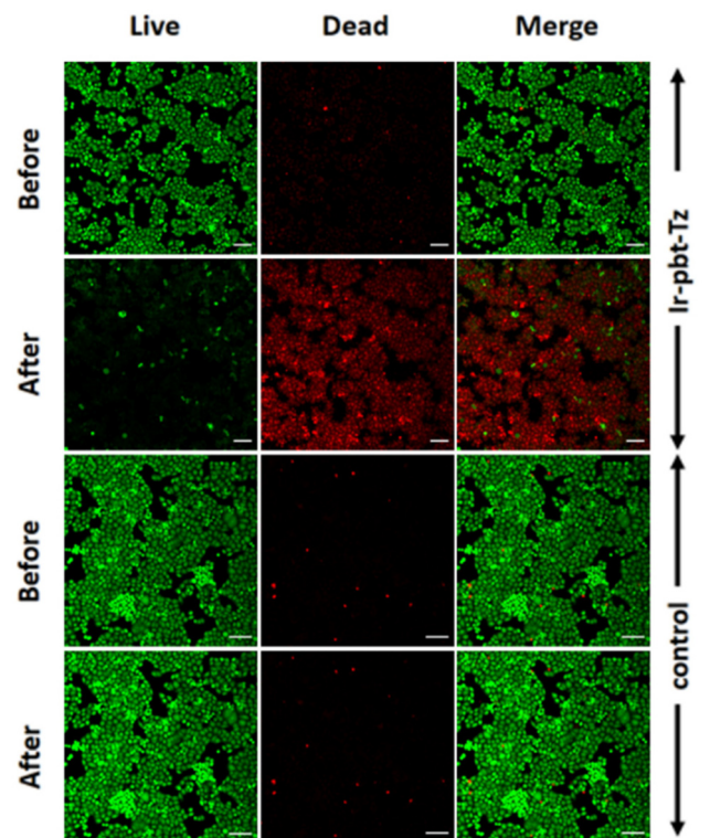
Fig. 4 Fluorescence microscopy images of A549 cells upon incubation with Ir-pbt-Tz (50 nM) for 4 h and calcein-AM (live cells, green, 0.5 \mu\text{M} , \lambda_{\text{ex}} = 488 \text{ nm} , \lambda_{\text{em}} = 510\text{--}540 \text{ nm} )/EthD-1 (dead cells, red, 2 \mu\text{M} , \lambda_{\text{ex}} = 530 \text{ nm} , \lambda_{\text{em}} = 640\text{--}670 \text{ nm} ) in the dark or upon irradiation ( 740 \text{ nm} , 6 \text{ J cm}^{-2} ). Scale bar: 100 \mu\text{m} .
