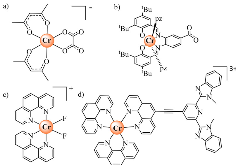
Scheme 1 Kinetically-inert heteroleptic six-coordinate \text{Cr}^{\text{III}} complexes used as complex-as-ligand when preparing multimetallic assemblies. 12,18–21
