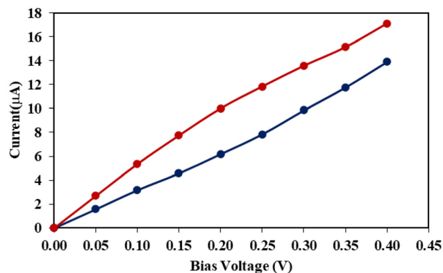
Fig. 5 Calculated current versus applied bias voltage on R_{sulf} (blue) and C_{60}@R_{sulf} (red) molecular junctions.
