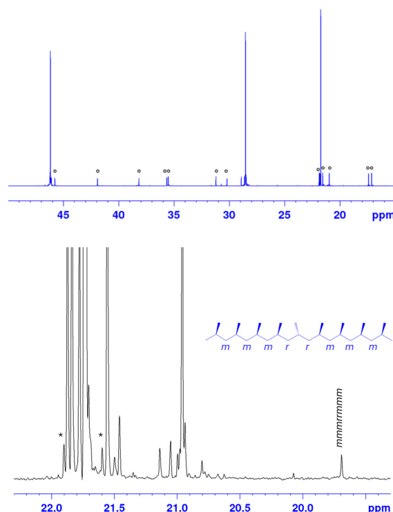
Fig. 2 Full 13 C NMR spectrum (top) and expansion of the methyl region (bottom) of highly regioirregular iPP made using catalyst Ty7 . Peaks marked with * and o are due 13 C– 13 C satellite band and to regioerrors, respectively.
