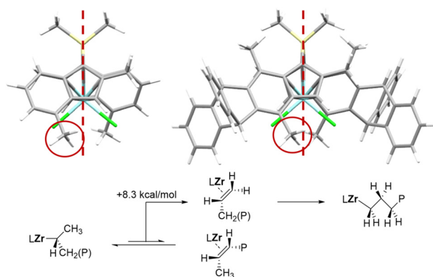
Fig. 3 Top: change in relative orientation of the indenyl fragments upon repositioning the 4-Me substituents. Comparison of rac -Me 2 Si(2-Me-4-Me-indenyl) 2 ZrCl 2 and Ty7 . The resulting interference with 1,2 transition states is responsible for the low regioselectivity of Ty7 . Red dashed lines indicate the middle plane of the active pocket, separating the two active sites. Bottom: the two possible \beta -hydrogen eliminations after 2,1 insertion in Ty7 .
