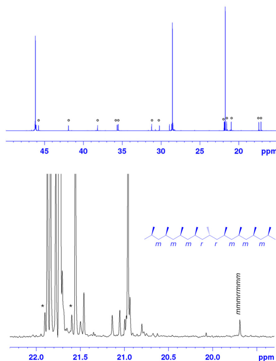
Fig. 2 Full 13 C NMR spectrum (top) and expansion of the methyl region (bottom) of highly regioirregular iPP made using catalyst Ty7 . Peaks marked with * and o are due to 13 C– 13 C satellite band and to regioerrors, respectively.
