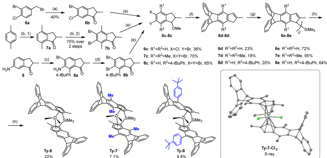
Scheme 2 Syntheses of 5,6-bridged triptycene precatalysts: (a) 1. MeCH(COOEt) 2 , NaOEt, EtOH 2. KOH, water, reflux; 3. 180 °C; 4. SOCl 2 , CH 2 Cl 2 ; 5. AlCl 3 , CH 2 Cl 2 . (b) 1. AlCl 3 , CH 2 Cl 2 ; 2. one-pot: Br 2 , CH 2 Cl 2 . (c) 1. NBS, DMF; 2. 4- t BuPhB(OH) 2 , Cs 2 CO 3 , Pd(PPh 3 ) 4 , dioxane/water, reflux; 3. NBS, DMF. (d) amyl nitrite, CuBr 2 , MeCN. (e) 1. NaBH 4 , MeOH-THF; 2. for 6c , 7c : KOH, MeI, DMSO; for 8c : NaH, MeI, THF. (f) 1. n BuLi, THF, anthracene, 2. for 6d : HCl (aq.), MeOH, reflux; for 7d , 8d : TsOH, PhMe, reflux. (g) For 6e , 7e : i. n BuLi, Et 2 O, ii. THF, CuCN, Me 2 SiCl 2 ; for 8e : i. n BuLi, Et 2 O, ii. Me 2 SiCl 2 , N -methylimidazole (h) i. n BuLi, ZrCl 4 , Et 2 O; 3. MeMgBr, Et 2 O. Insert: crystal structure of Ty7-Cl 2 ; image generated by Mercury software with thermal ellipsoids at 50% probability level; hydrogen atoms and co-crystallized toluene molecules omitted for clarity.
