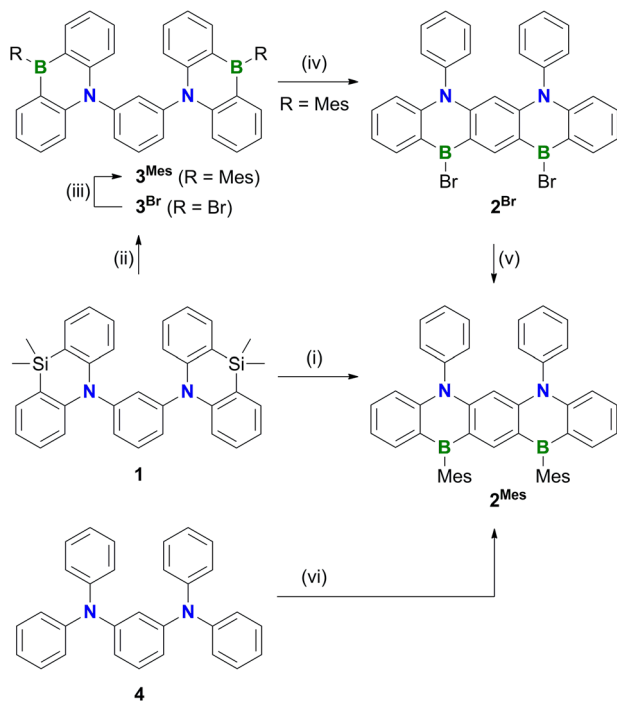
Scheme 2 Synthetic pathways to 2^{Mes} . Conditions: (i) 1. BBr_3 (12 equiv.), C_6H_6 , 180 °C, 116 h, sealed ampoule; 2. MesMgBr (3 equiv.), toluene, -78 °C to room temperature, 39% over two steps; (ii) BBr_3 (5 equiv.), CH_2Cl_2 , room temperature, 1 d, closed J. Young vessel, product was used after solvent exchange without further purification; (iii) MesMgBr (3 equiv. relative to 1 ), toluene, -78 °C to room temperature, 42% over two steps; (iv) BBr_3 (12 equiv.), C_6H_6 , 180 °C, 92 h, sealed ampoule, product was used after solvent exchange without further purification; (v) MesMgBr (3 equiv. relative to 3^{Mes} ), toluene, -78 °C to room temperature, 44% over two steps; (vi) 1. BBr_3 (12 equiv.), o -dichlorobenzene, 180 °C, 112 h, sealed ampoule; 2. MesMgBr (3 equiv.), toluene, -78 °C to room temperature, 58% over two steps.
